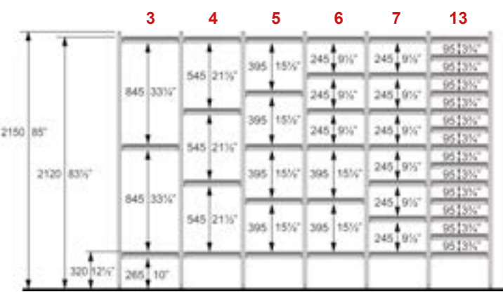
Shelf height: 2150 mm (85") / Room height > 2400 mm (95")
