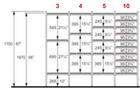
Shelf height: 1700 mm (67") / Room height > 1950 mm (77")
