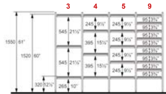
Shelf height: 1550 mm (61") / Room height > 1700 mm (67")
