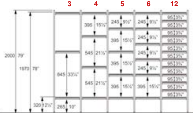
Shelf height: 2000 mm (79") / Room height > 2250 mm (89")
