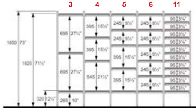
Shelf height: 1850 mm (73") / Room height > 2100 mm (83")
