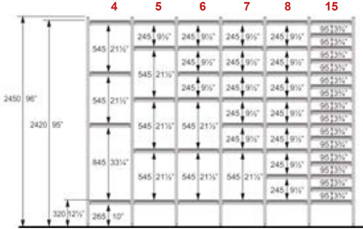
Shelf height: 2450 mm (96") / Room height > 2800 mm (110")
